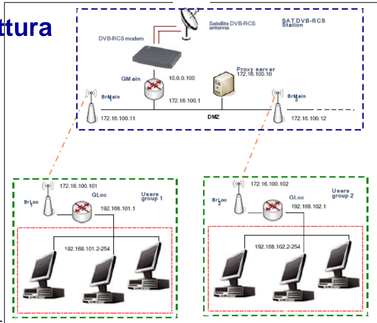
Fig. 1 - network architecture
